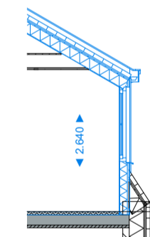
Dakkapel
